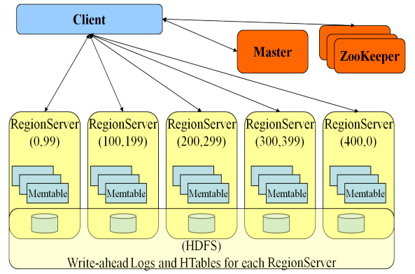
Figure 3: HBase architecture.
