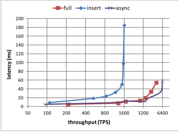
Figure 8: Read performance.
