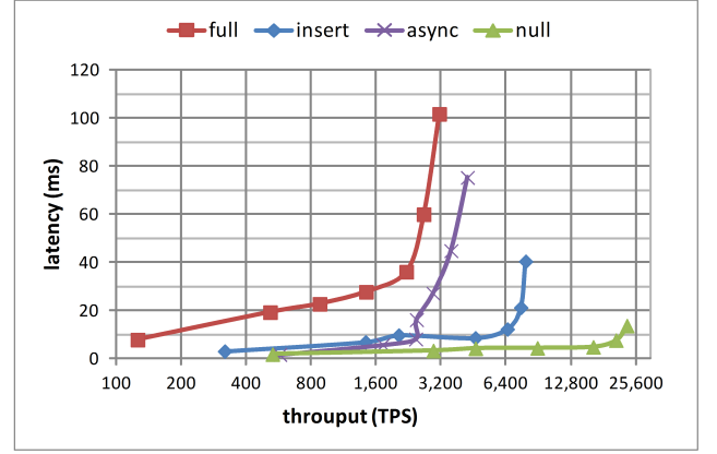
Figure 7: Update performance.
